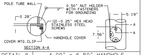
DETAIL 8 4.00" x 6.50" HANDHOLE
