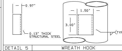
DETAIL 5 WREATH HOOK
