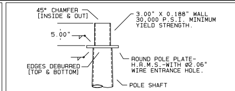
DETAIL 1 POLE TOP TENON
