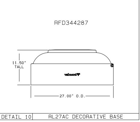
DETAIL 10 RL27AC DECORATIVE BASE
