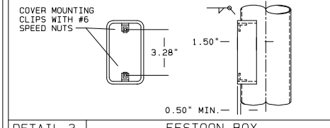
DETAIL 3 FESTOON BOX
