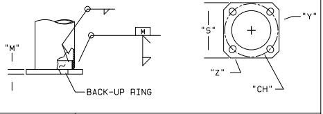
DETAIL 9 POLE BASE
