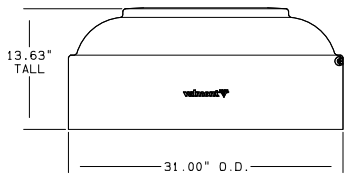
DETAIL 11 RL31AC DECORATIVE BASE
