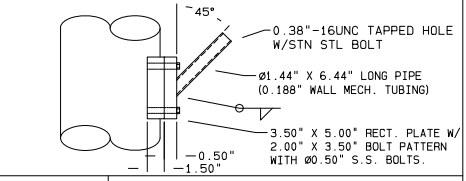
DETAIL 7 FLAG HOLDER
