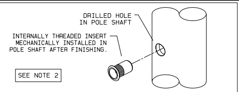
DETAIL 6 TYPICAL RIVNUT DETAIL
