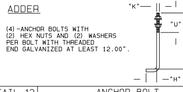
DETAIL 12 ANCHOR BOLT
