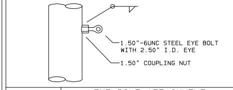
DETAIL 2 EYE BOLT ATTACHMENT
